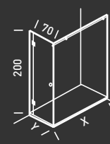
hinged door and fixed long side glass panel corner version
