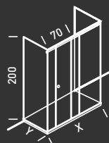
sliding door and fixed glass panels centre-of-the-wall version
